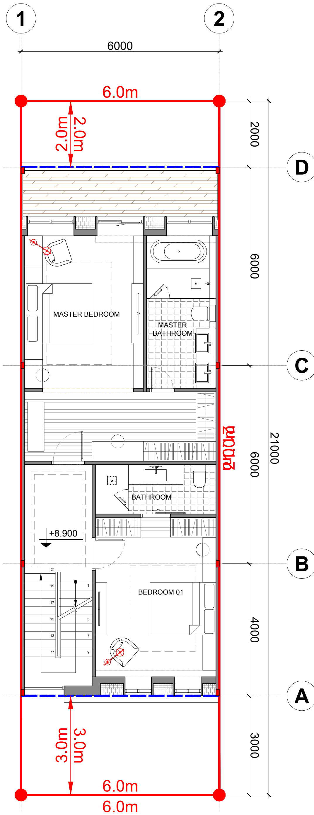
LEVEL 3 FLOOR PLAN
