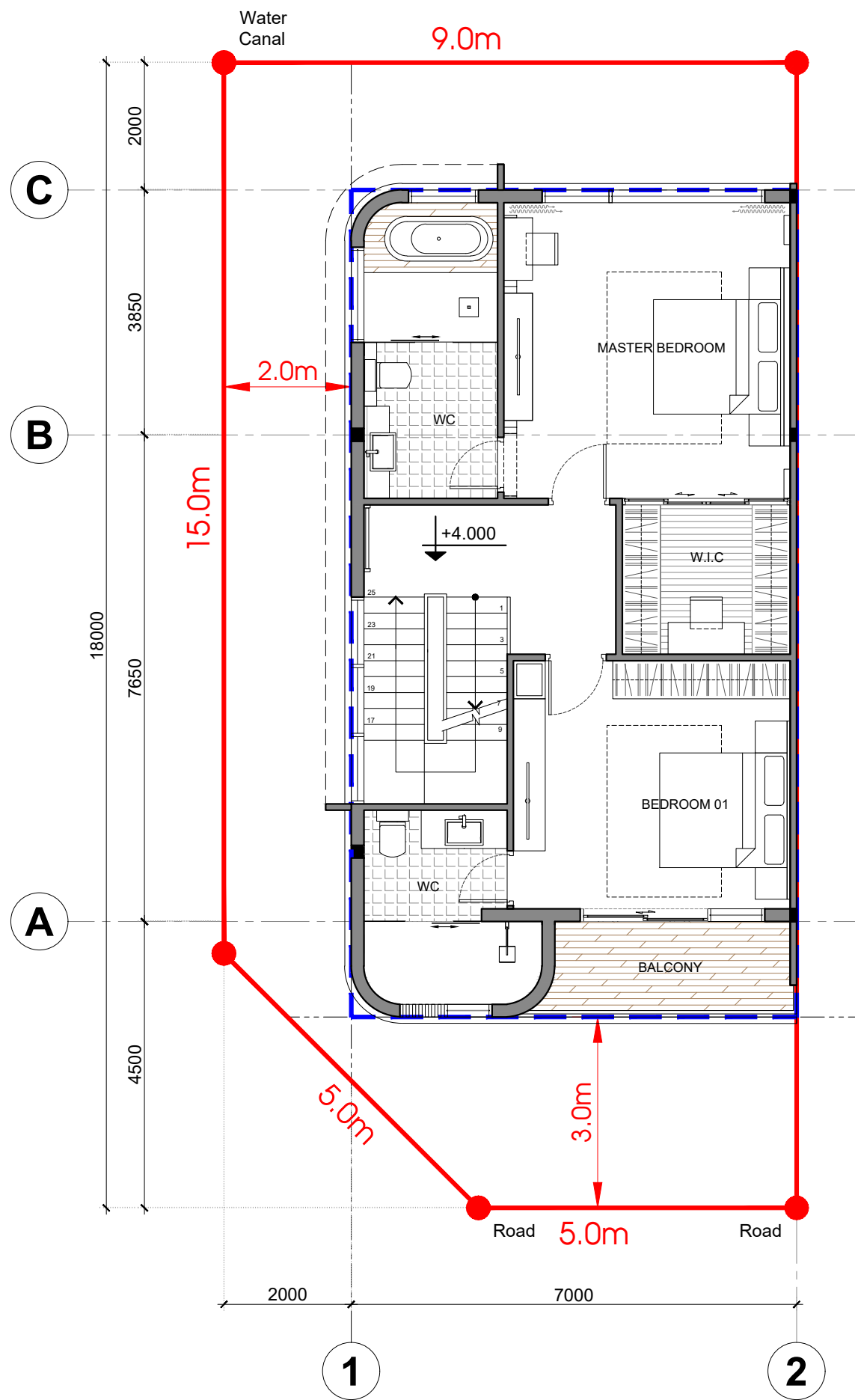
LEVEL 2 FLOOR PLAN
