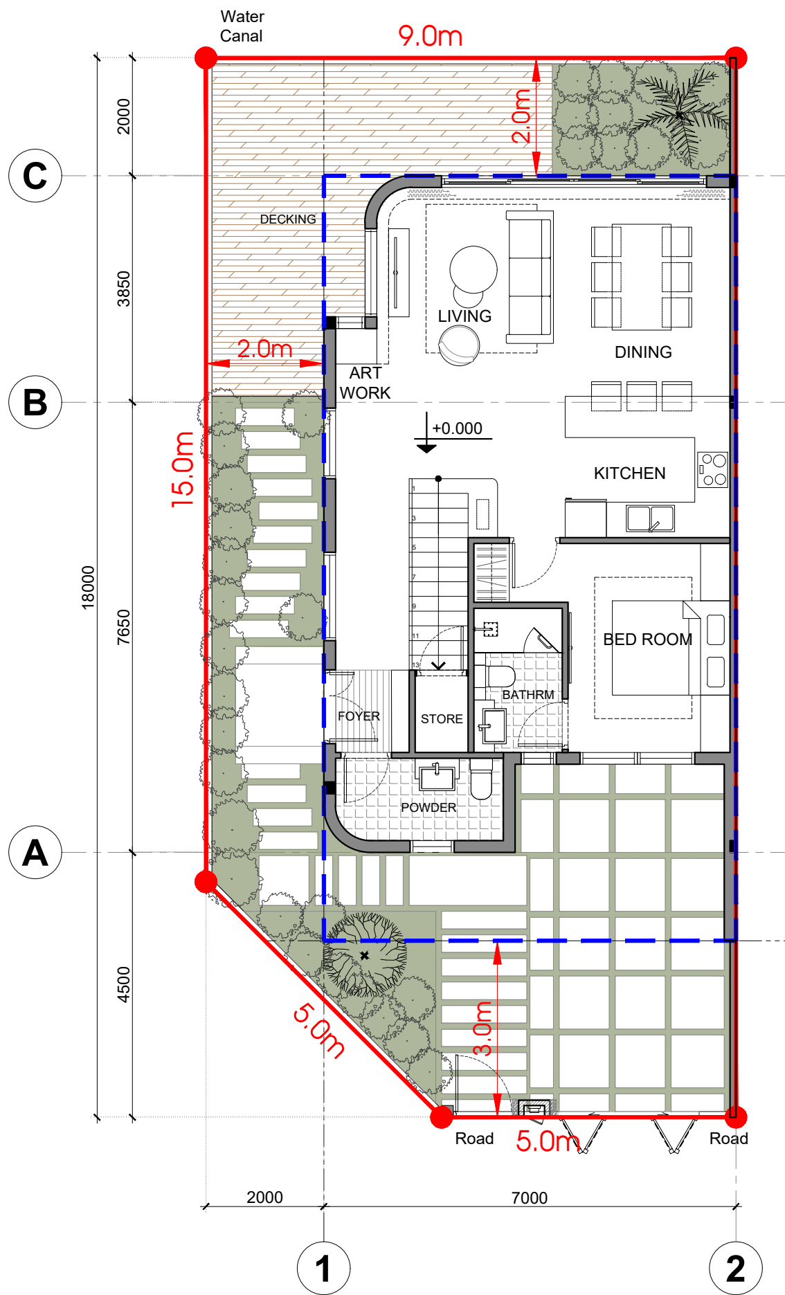
LEVEL 1 FLOOR PLAN
