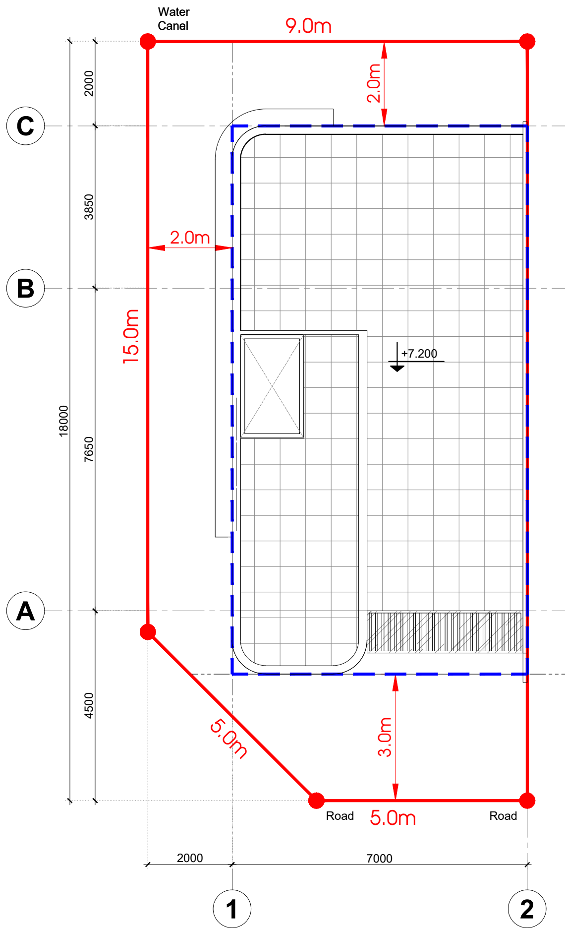
ROOF FLOOR PLAN
