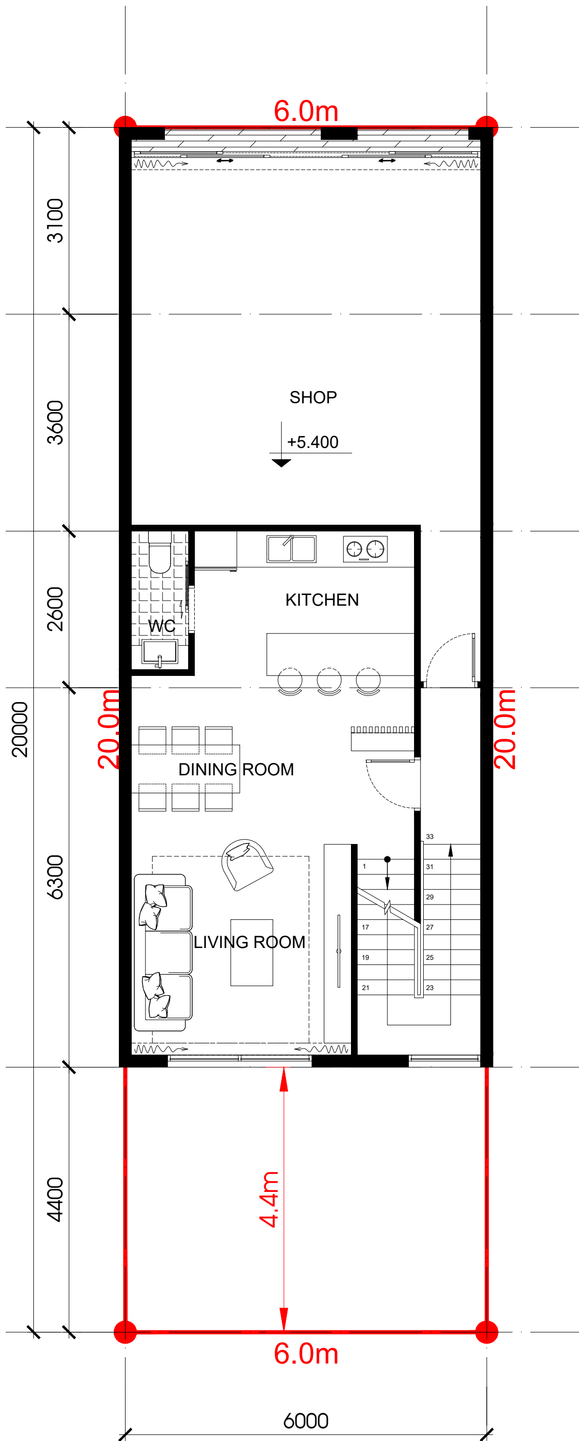
LEVEL 2 FLOOR PLAN
