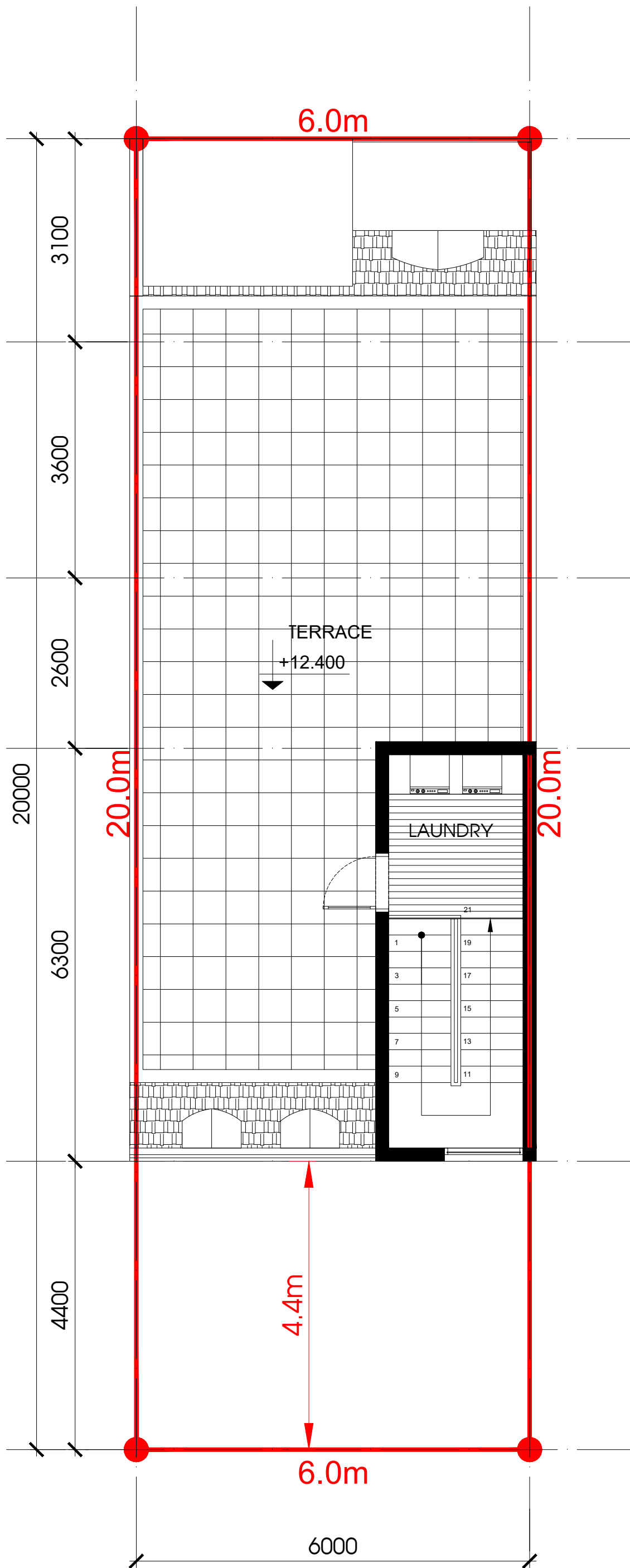
ROOF TERRACE PLAN
