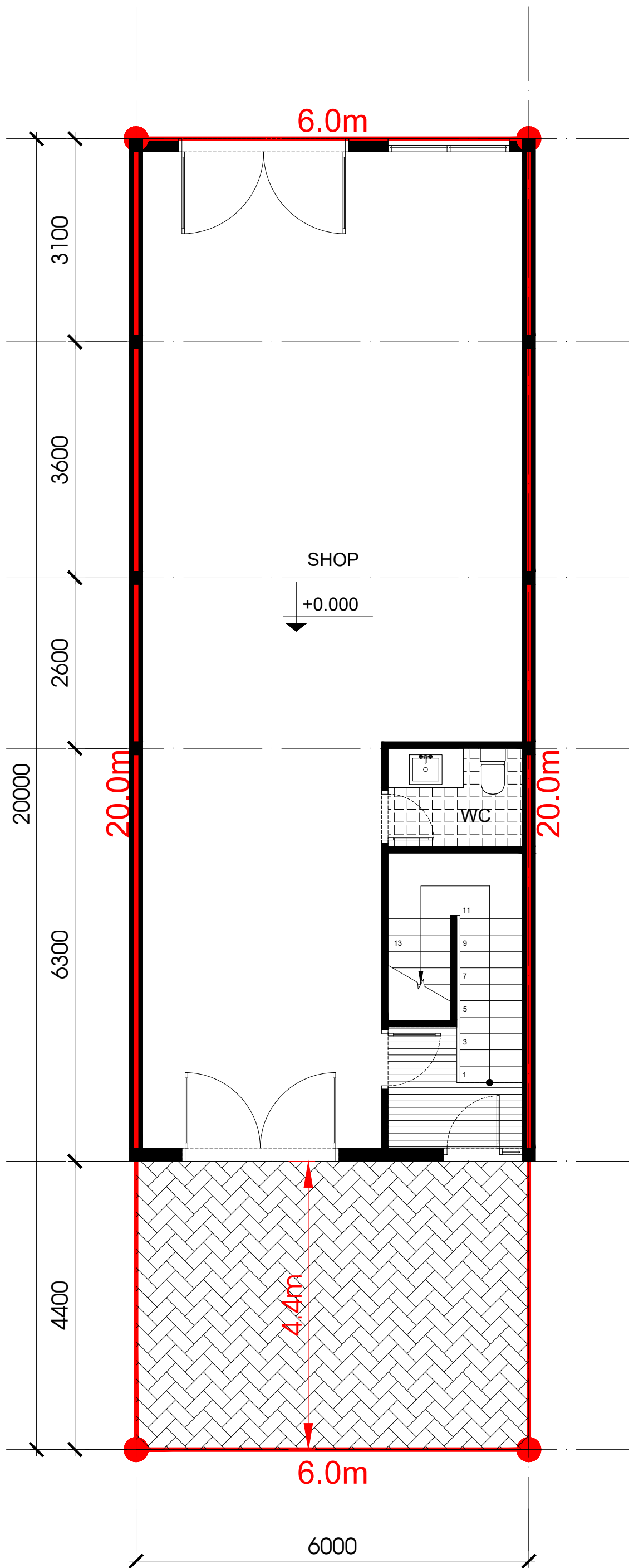
LEVEL 1 FLOOR PLAN
