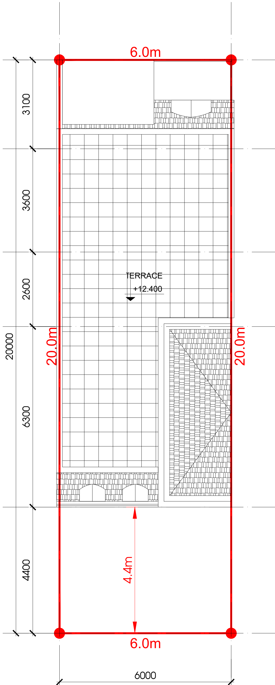
ROOF PLAN
