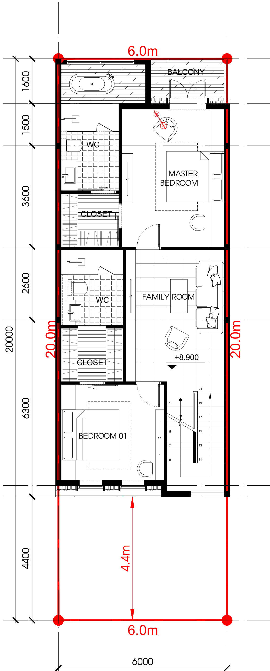
LEVEL 3 FLOOR PLAN
