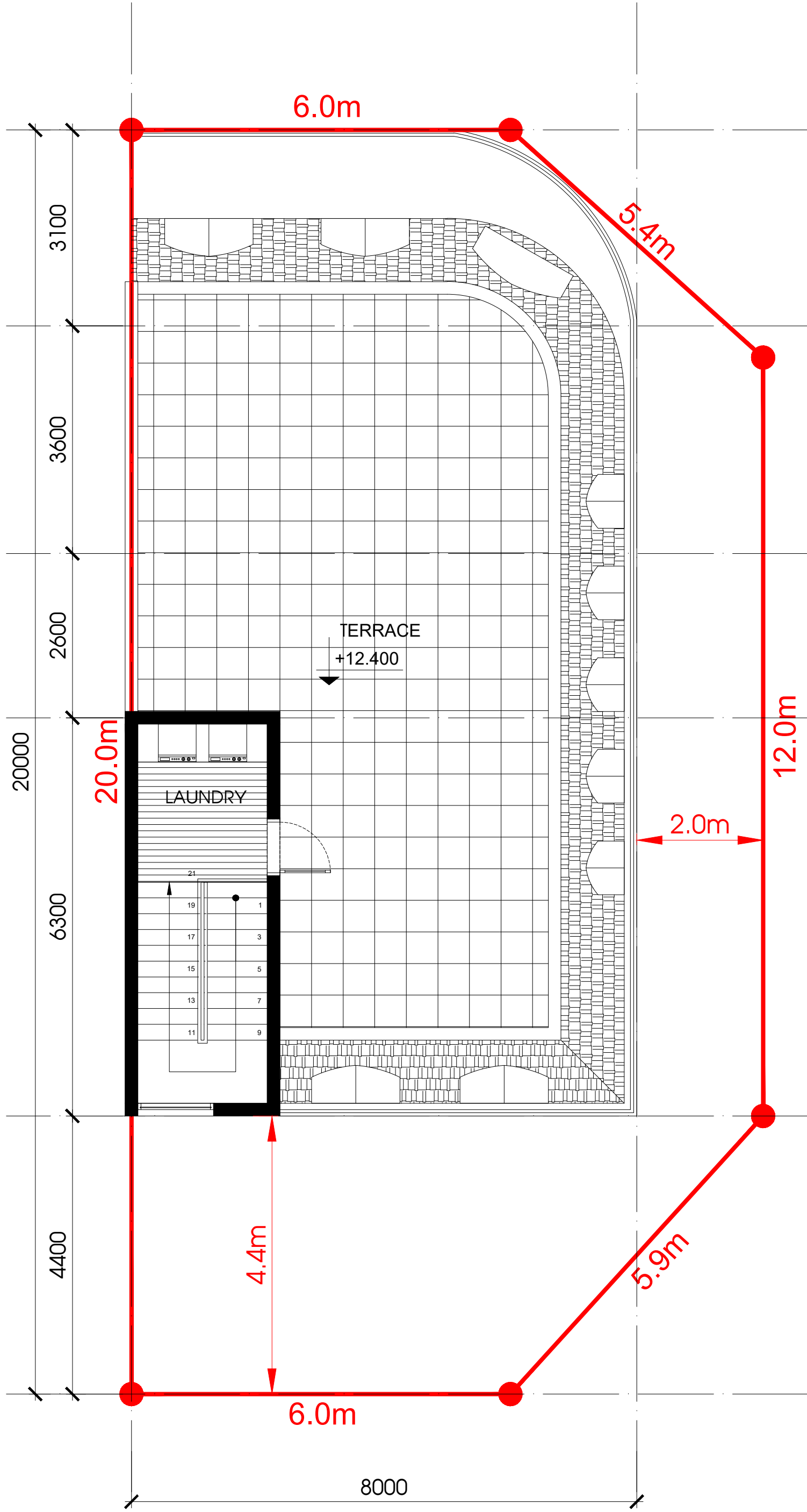
ROOF TERRACE PLAN
