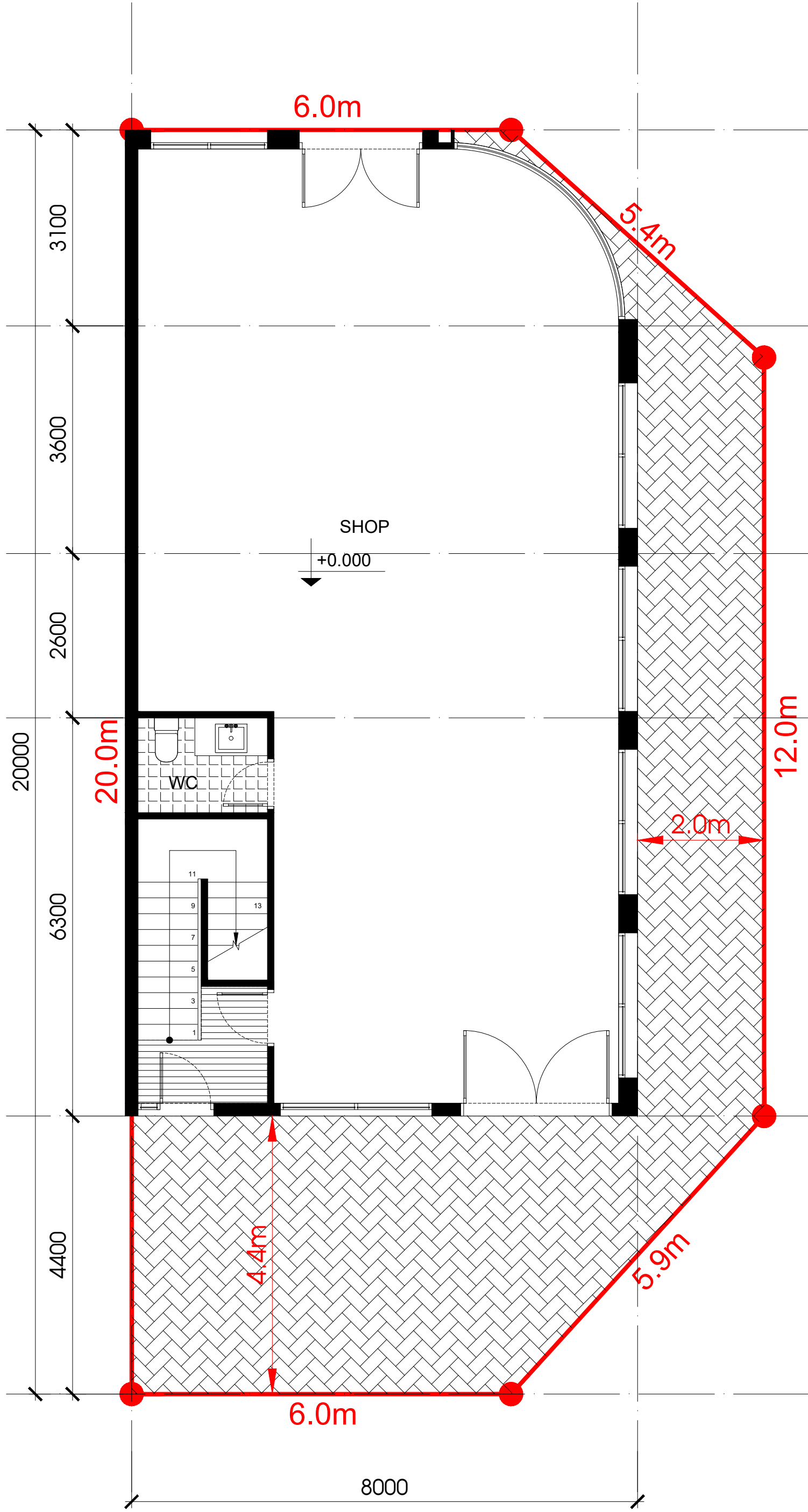
LEVEL 1 FLOOR PLAN
