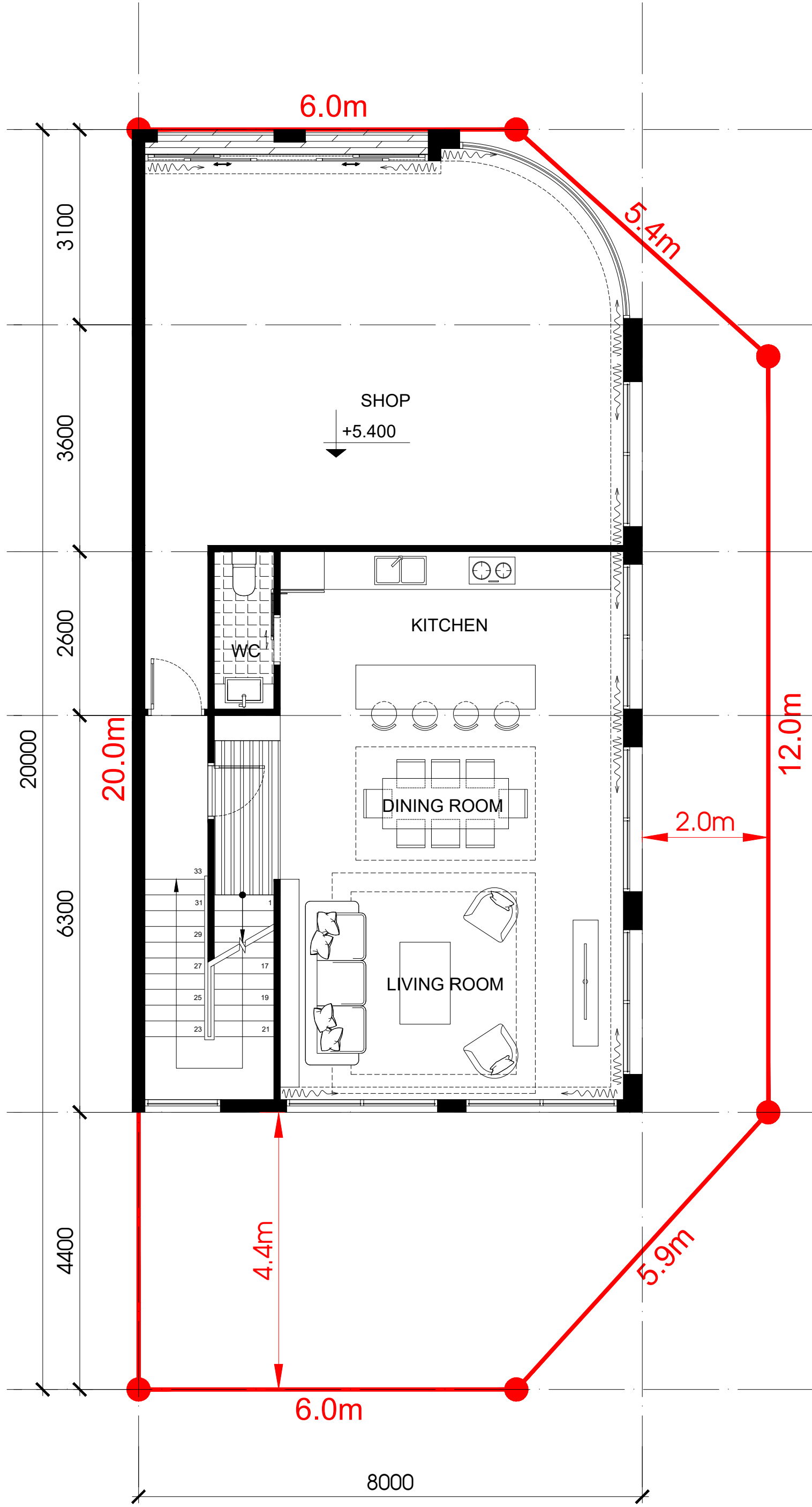
LEVEL 2 FLOOR PLAN
