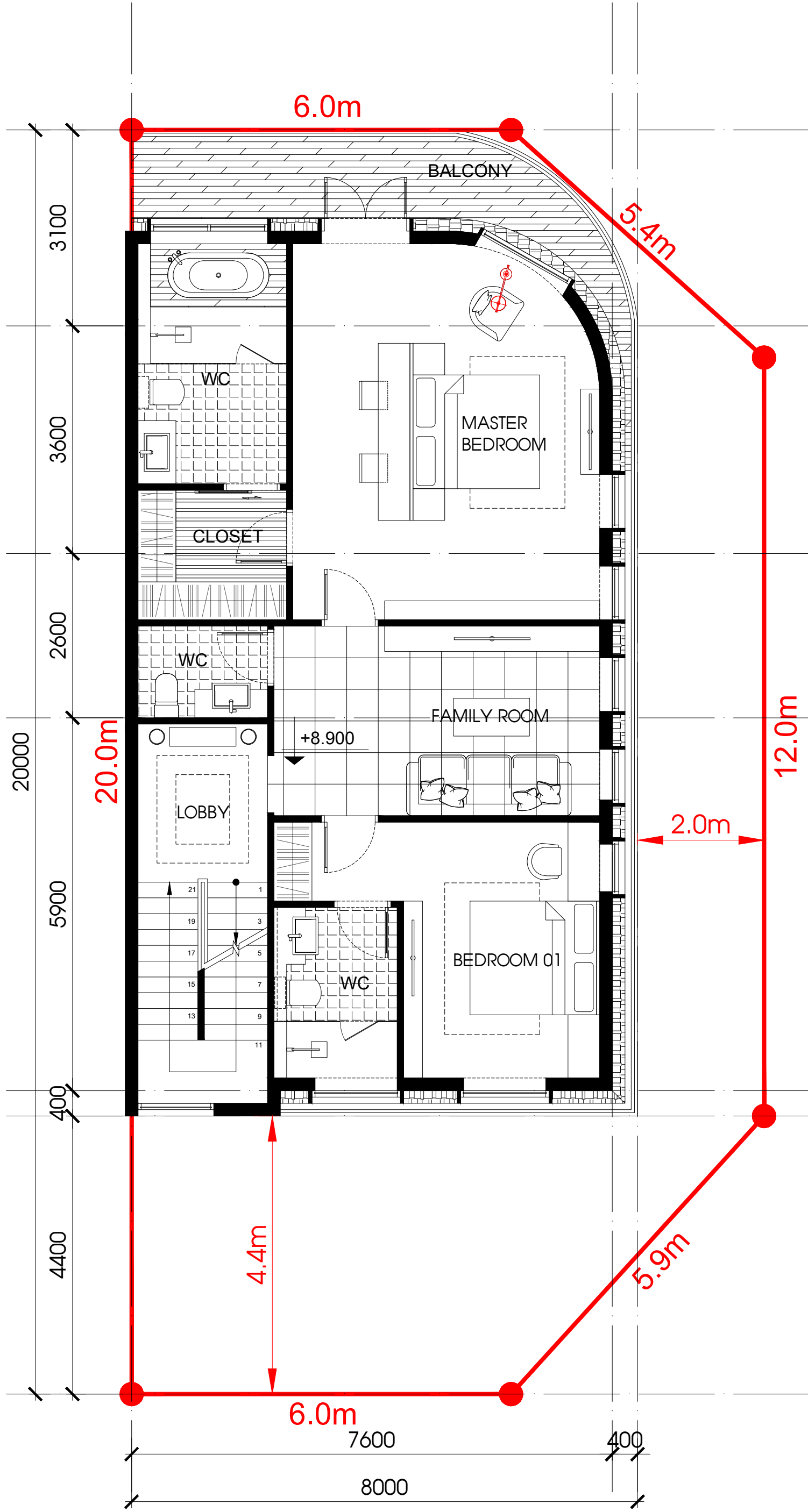
LEVEL 3 FLOOR PLAN
