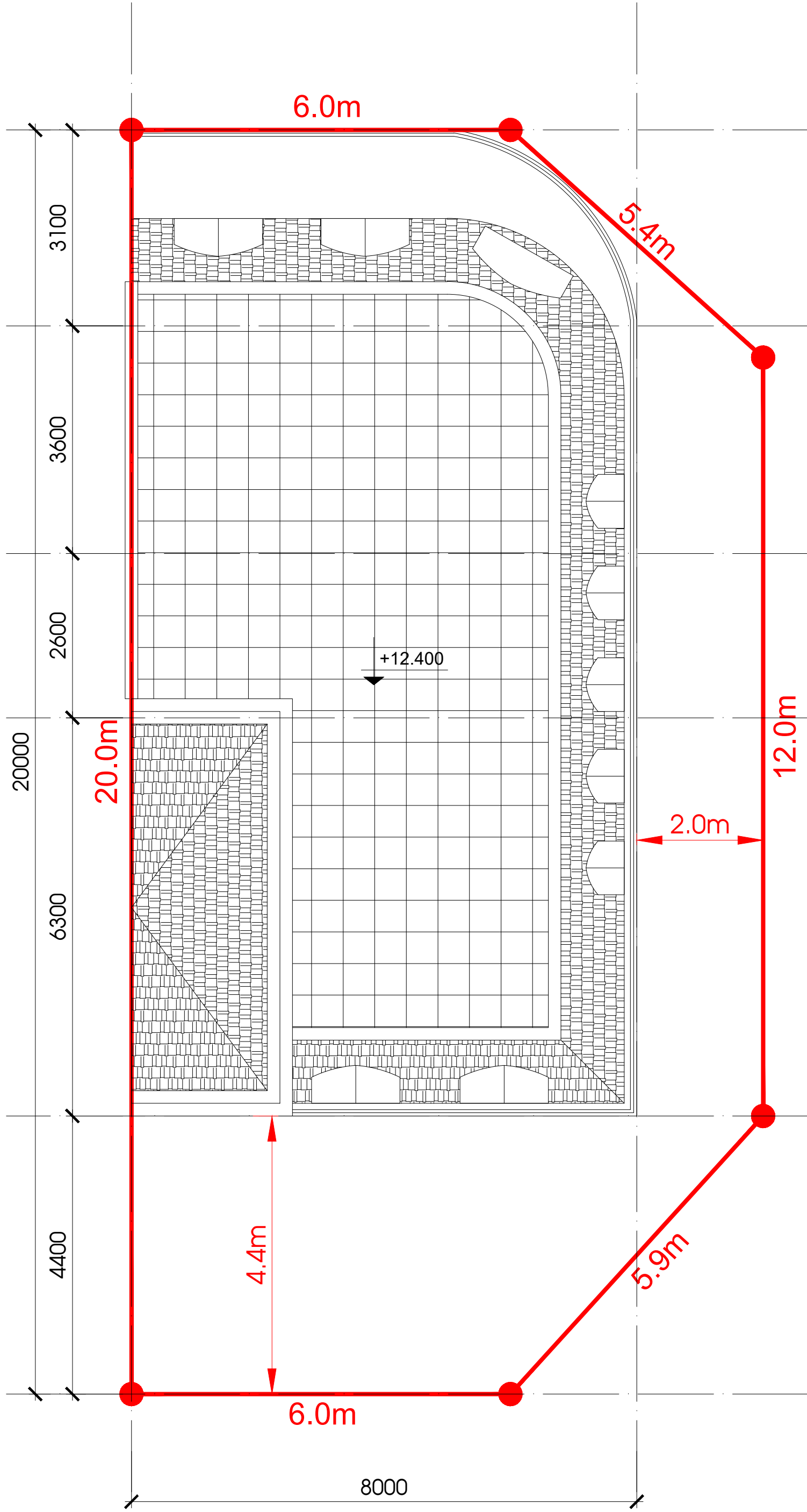
ROOF PLAN
