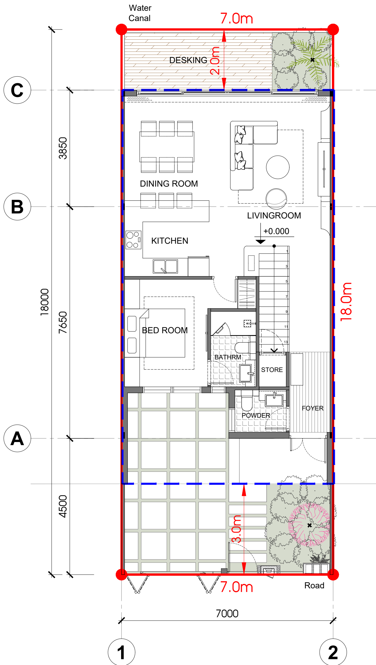
LEVEL 1 FLOOR PLAN
