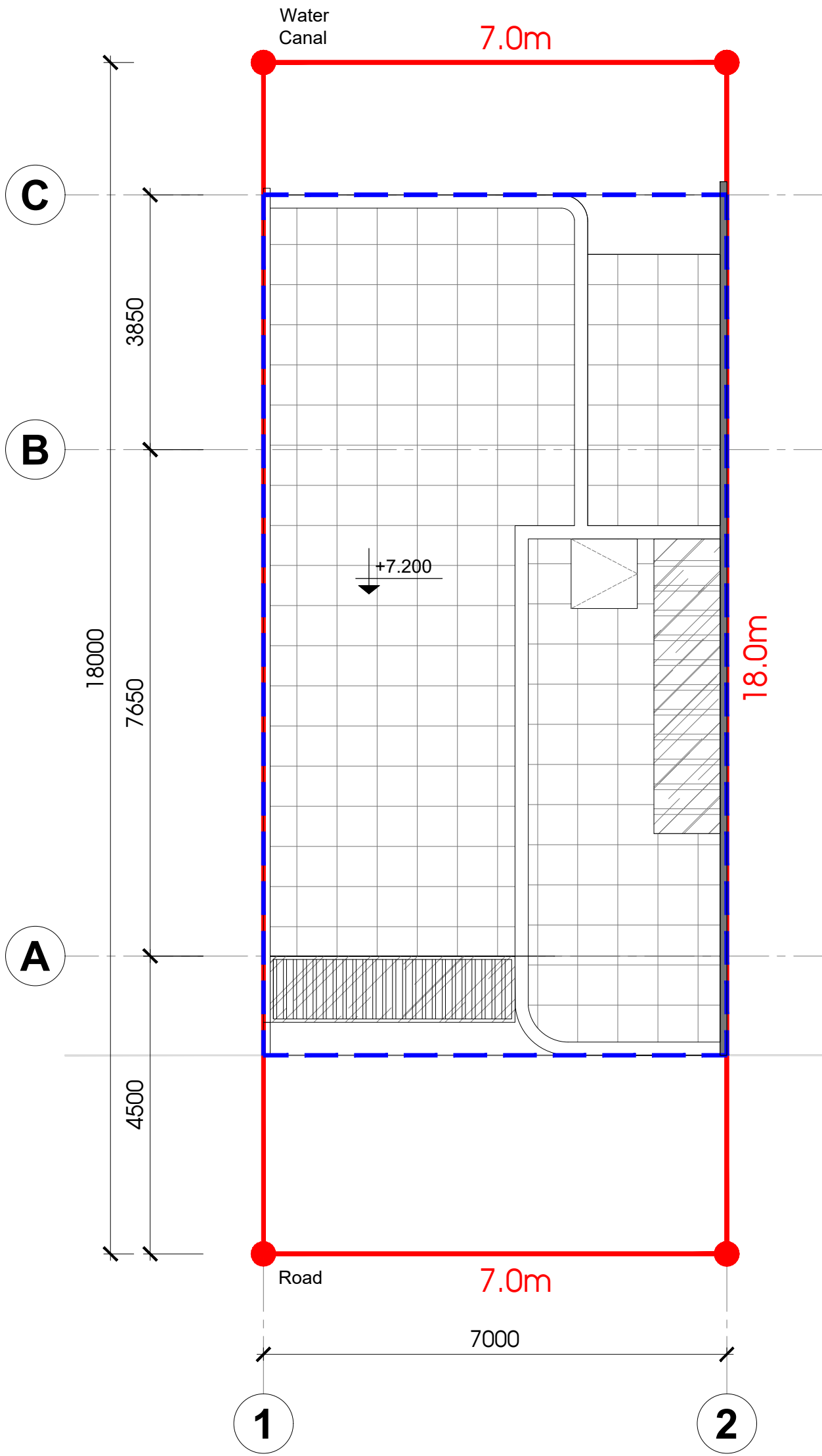
ROOF TERRACE PLAN
