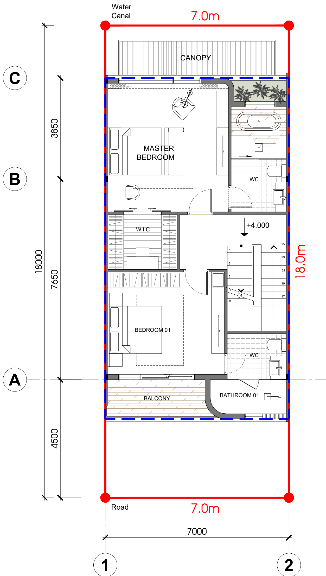
LEVEL 2 FLOOR PLAN
