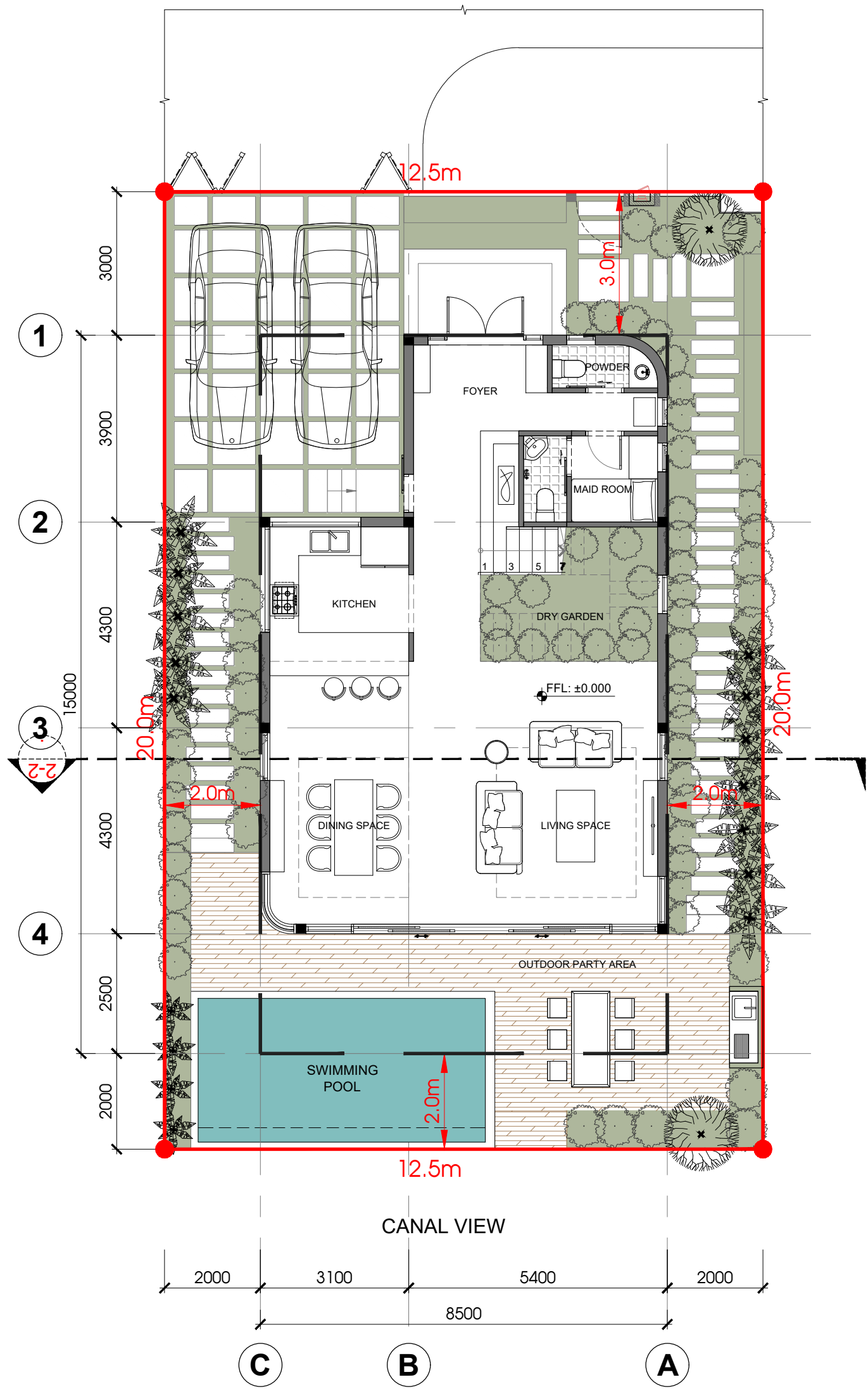
LEVEL 1 FLOOR PLAN
