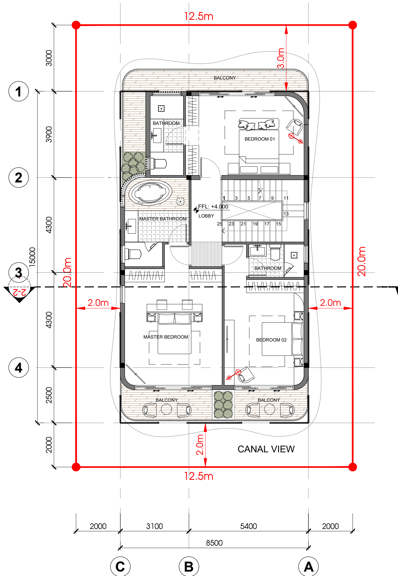
LEVEL 2 FLOOR PLAN
